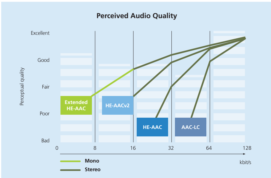
Figure 4: Qualitative illustration of perceived audio quality.
