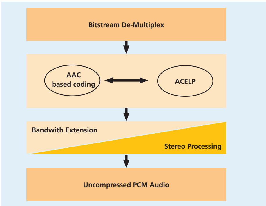
Figure 2: Working principle of the Extended HE-AAC core decoder.
