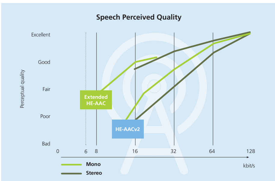
Figure 5: Speech perceived quality. From ISO/IEC JTC1/SC29/WG11 USAC Verification Test Report.
