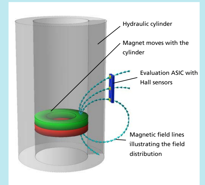
Example for linear positioning at cylinders
