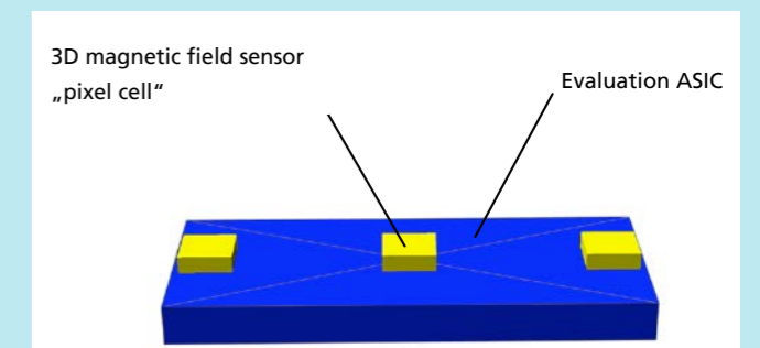
Schematic structure of the evaluation ASIC with three integrated magnetic pixel cells
